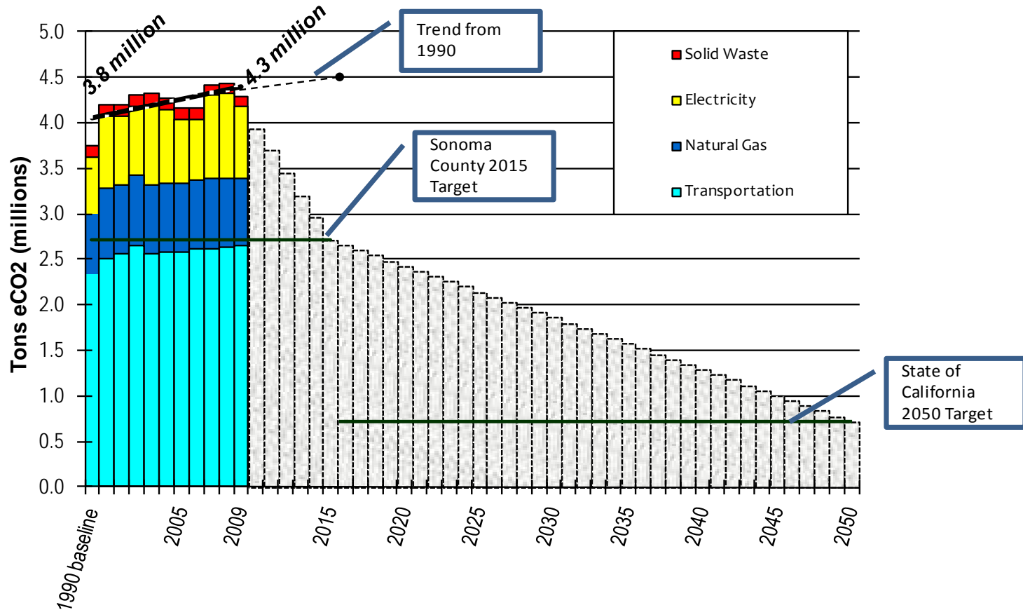
Sonoma County Total GHG Emissions Solid Waste, Electricity, Natural Gas and Transportation Updated 2010
